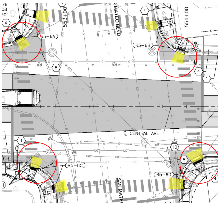
Figure 27: Central Ave and San Mateo Roadway Plan (Source: ABQ Ride Feb 2016 construction plans sheet 81 or 261)
