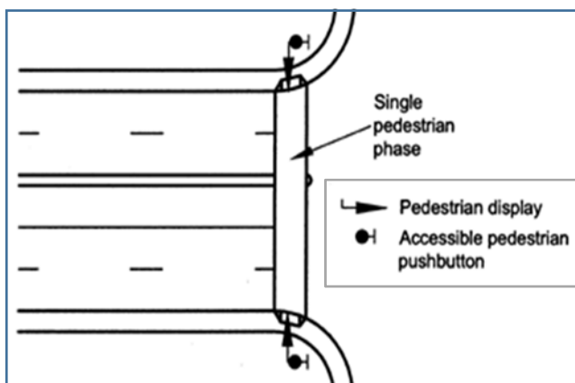
Figure 29: One-stage pedestrian crossing with median refuge island (Source: FHWA, Publication FHWA-HRT-04-091)
