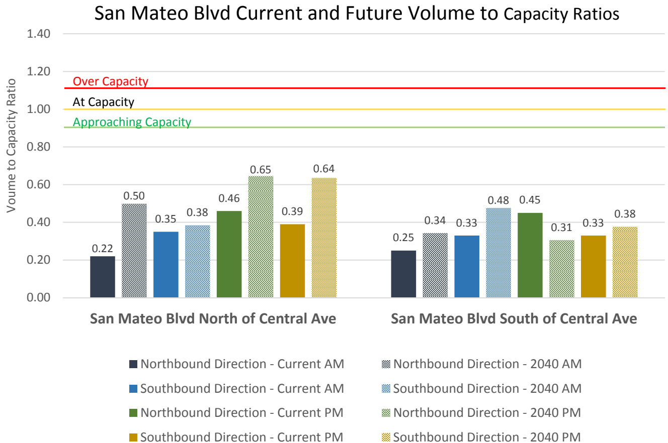
Chart 1: San Mateo Blvd current and future volume to capacity ratios (Source: MRCOG)
