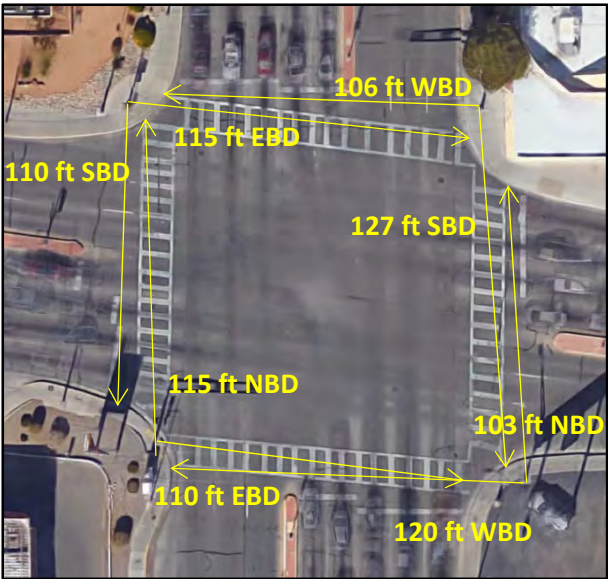
Figure 10: Intersection Crossing Distances (Source: MRCOG)
